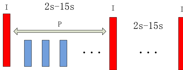
Figure 4 Dynamic GOP
