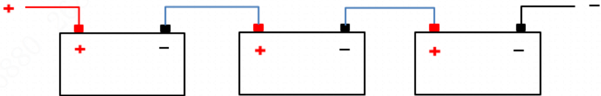
Series connection
