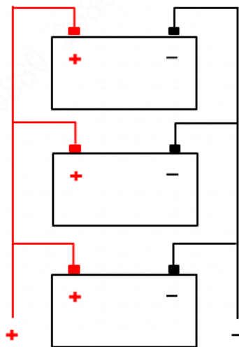
Parallel connection
